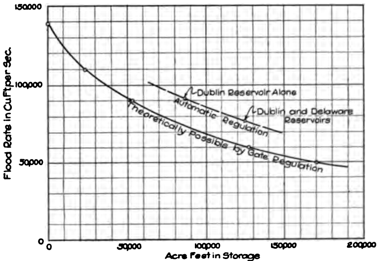
FIG. 43.—Diagram showing the effect of various storage volumes in the reduction of flood rates, Columbus flood of March, 1913.
